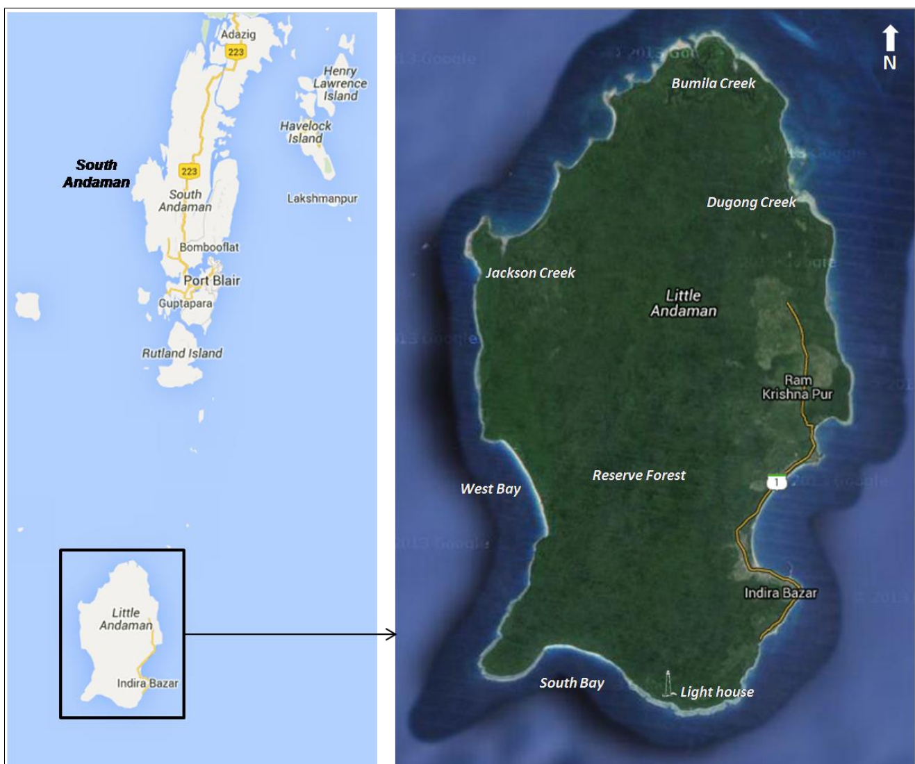
Figure 1. Location map of Little Andaman Island
